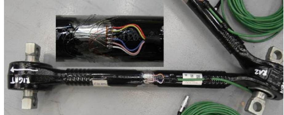
V杆应变测点布置
